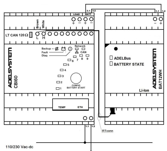
Fig. 3 –Connect to DC Ups
