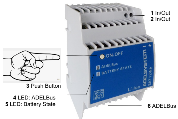
Fig. 2 –Battery Bank connections
