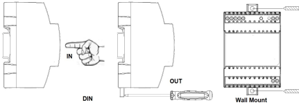
Fig. 1 – Mounting of the BAT12Wh
