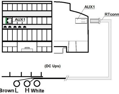
Fig. 4 –Connection RTConn cable
