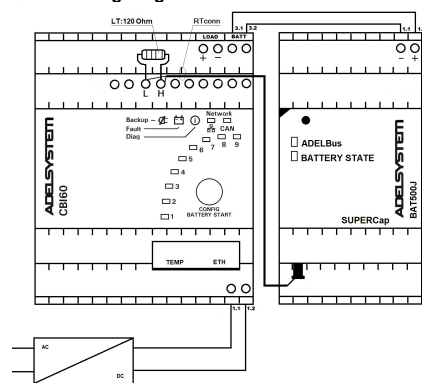
Fig. 3 –Connect to DC Ups
